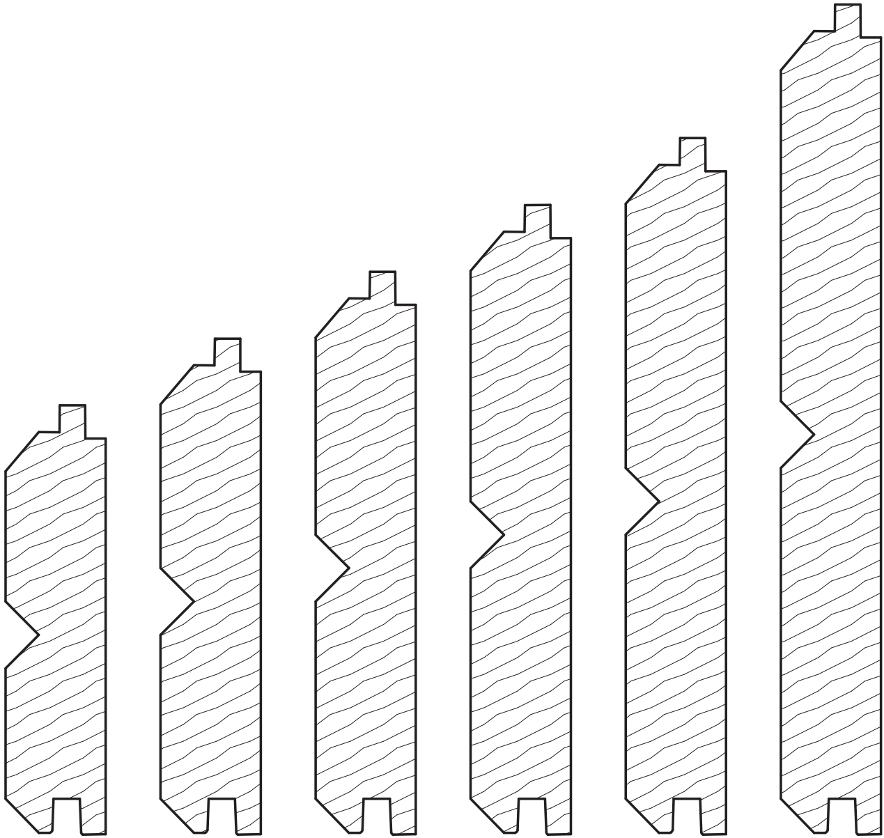
SEP-030 3/4 x 3
