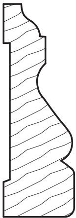
SEC-138 3/4 x 2-1/4
