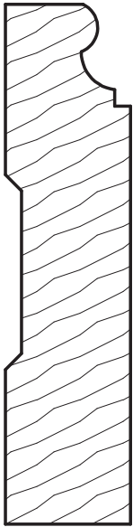
SEC-227 11/16 x 3
