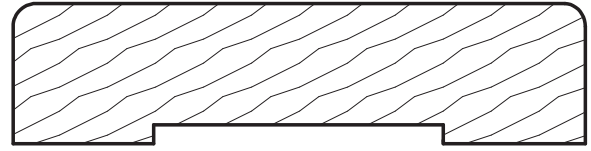
S4S-002 3/4 x 3
