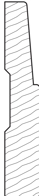
SEC-260 5/8 x 3-1/2
